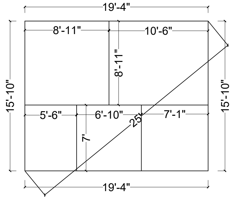
Center line Layout Plan
